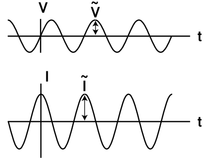
z / In a capacitor, the current is 90^\circ ahead of the voltage in phase.
